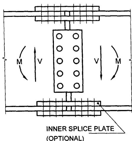
30A Conventional Splice (Typical)
