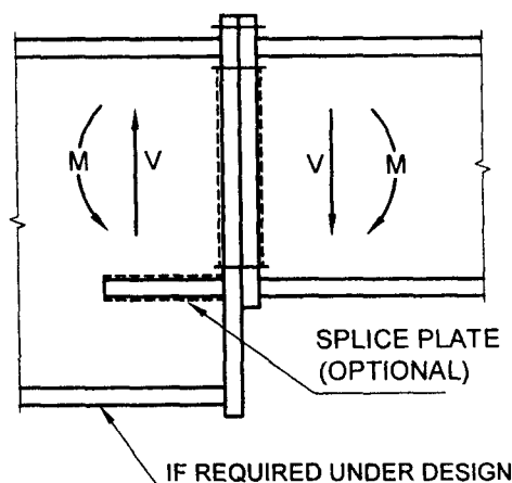
30B End Plate Splice
